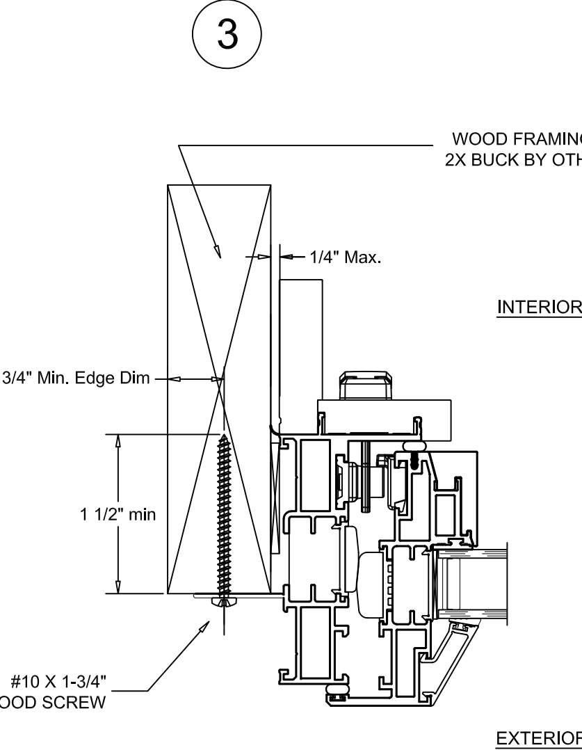
HORIZONTAL SECTION DETAIL
