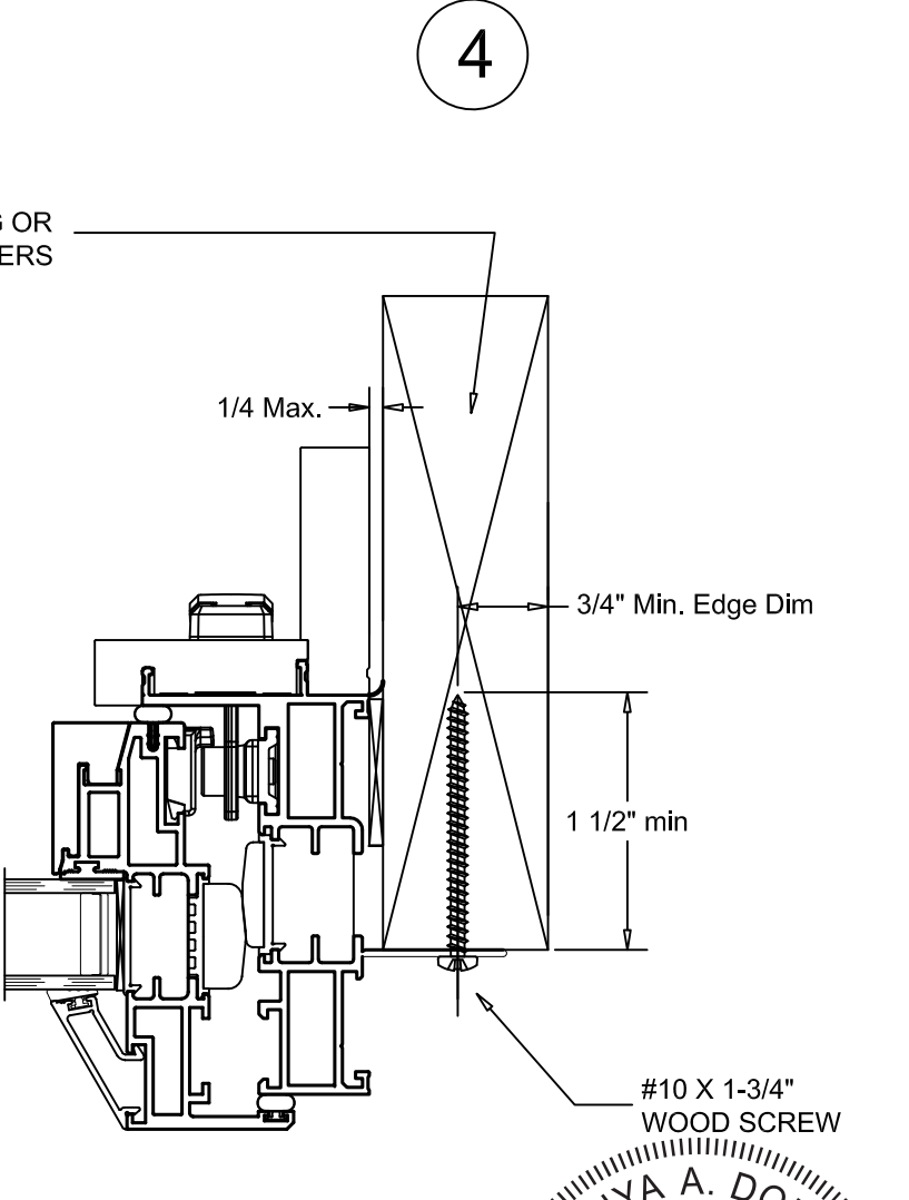
HORIZONTAL SECTION DETAIL
